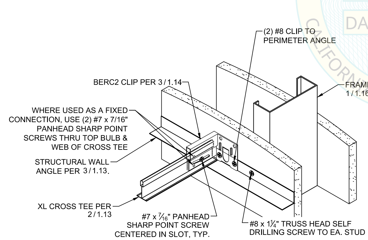
2 SLIP CONNECTION OF CROSS TEE TO WALL SCALE: N.T.S.
