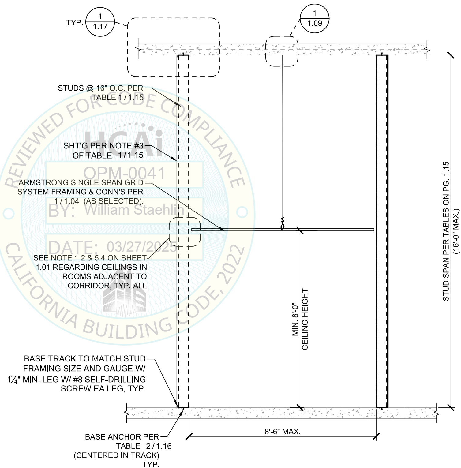
CORRIDOR SECTION
