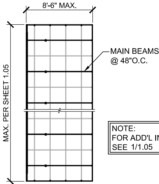
B CEILING LAYOUT B STRAIGHT W/ MAINS @ 48"O.C. (FOR S_{DS} \leq 1.50 ) SCALE: N.T.S.
