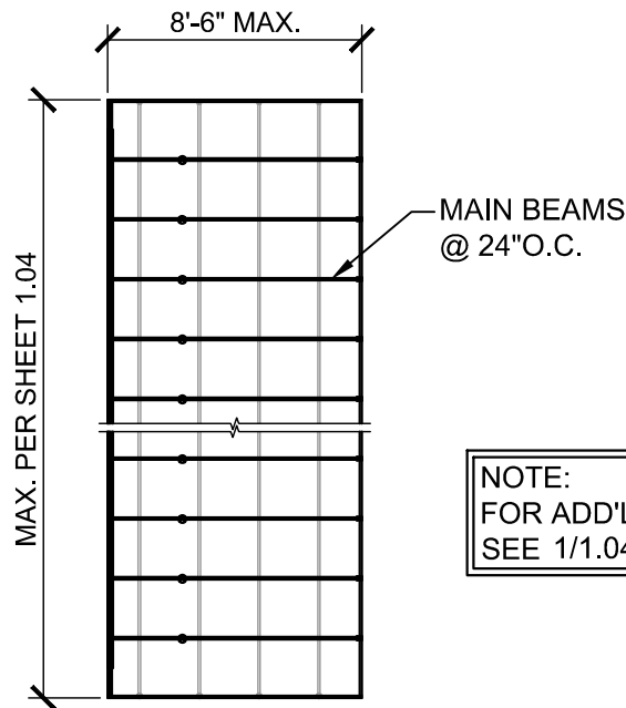
A CEILING LAYOUT A STRAIGHT W/ MAINS @ 24"O.C. (FOR S_{DS} \leq 1.83 ) SCALE: N.T.S.
