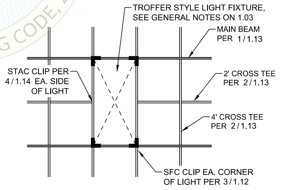
1 LIGHTS IN 4' O.C. MAIN BEAM LAYOUT SCALE: 3/8" = 1'-0"
