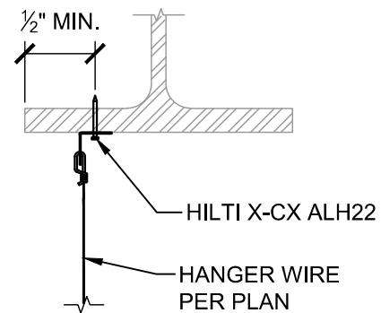
C HANGER WIRE @ STEEL BEAM
