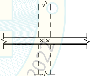
2 STRUCTURAL WALL ANGLE SPLICE SCALE: 1 1/2"=1'-0"
