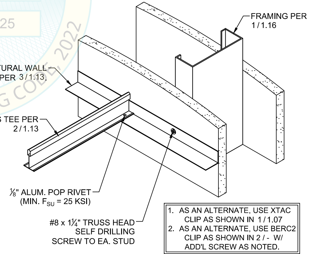
1 FIXED CONNECTION OF CROSS TEE TO WALL SCALE: N.T.S.
