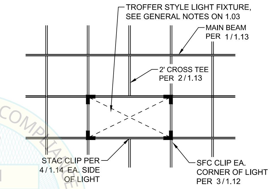
2 LIGHTS IN 2' O.C. MAIN BEAM LAYOUT SCALE: 3/8" = 1'-0"
