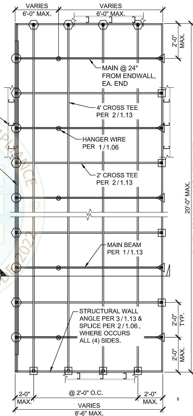
CEILING LAYOUT FOR STRAIGHT CORRIDOR W/ MAIN BEAMS @ 48"O.C. (FOR S_{DS} \leq 1.50 )
