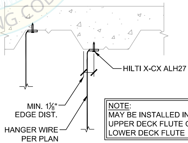
A HANGER WIRE @ CONCRETE FILLED METAL DECK
