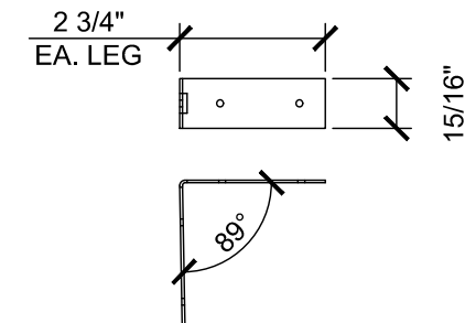
2 CROSSTEE ADAPTER CLIP (XTAC) - PART # XTAC SCALE: 3"=1'-0"
