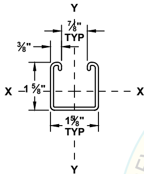
1 5/8 x 1 5/8 x 12ga SINGLE STRUT
