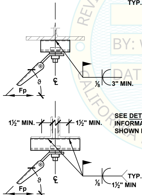
DETAIL C WELDING OPTION
