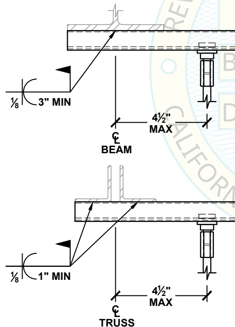
DETAIL C
