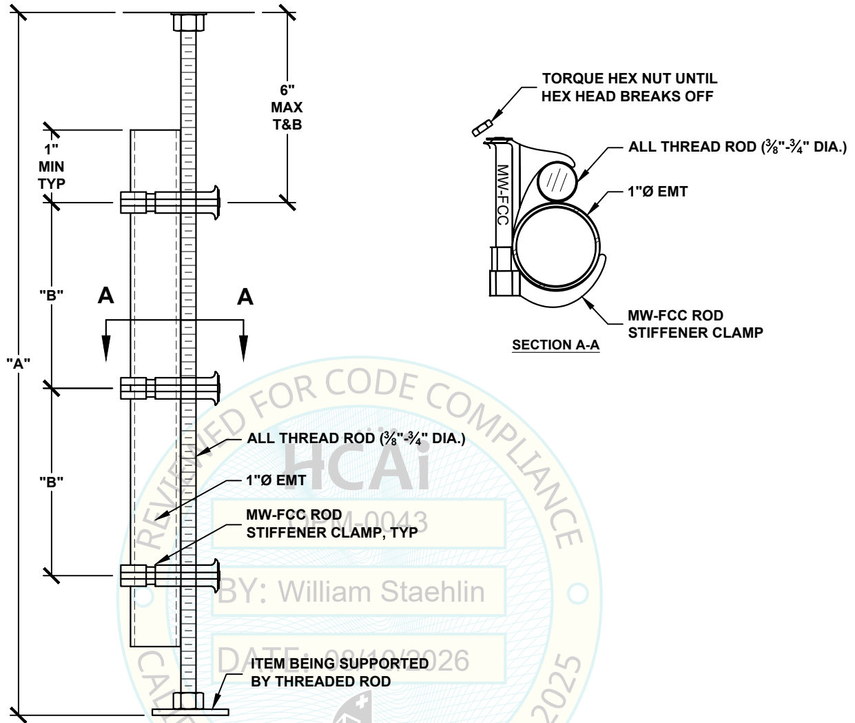
ROD STIFFENER CLAMP WITH EMT CONDUIT ASSEMBLY RATINGS (ASD)
