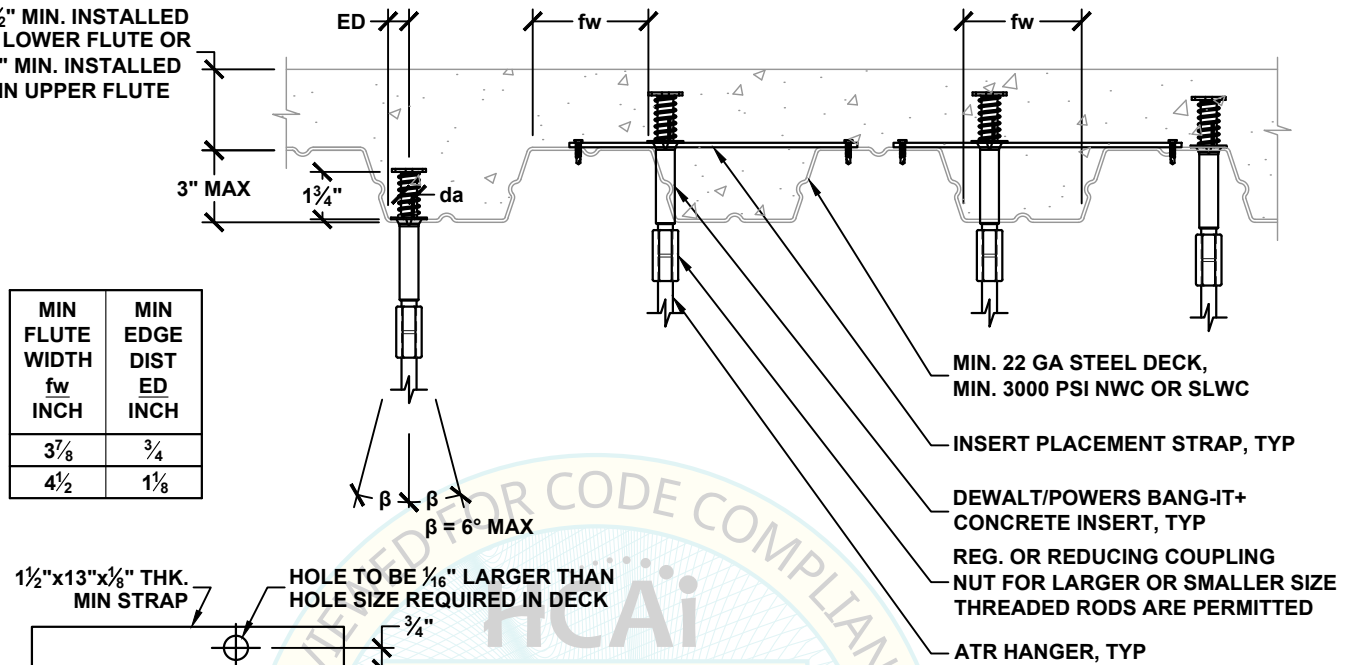
INSERT PLACEMENT STRAP
