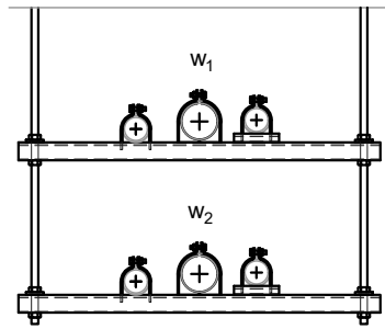
CASE 1 IF w_{total} < 10 LB/FT, NO BRACING REQ'D
