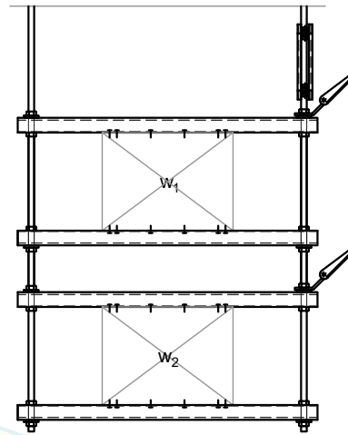
CASE 2 IF w_1 \geq 10 \text{ LB/FT} AND w_2 \geq 10 \text{ LB/FT} , BRACE EACH LAYER INDEPENDENTLY
