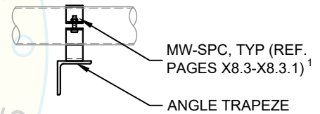
SIDE ELEVATION VIEW
