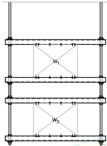
CASE 1 IF w_{total} < 10 \text{ LB/FT} , NO BRACING REQ'D
