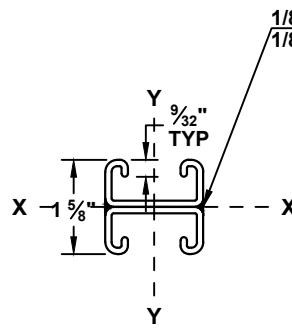
13/16 x 1 5/8 x 12ga DOUBLE STRUT
