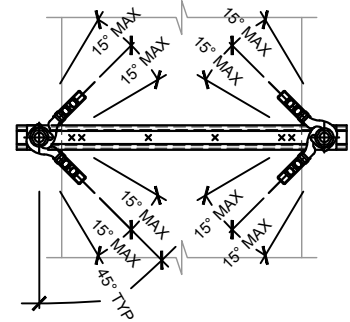
PLAN VIEW CABLE X-PATTERN BRACE INSTALLED IN-BETWEEN HANGERS
