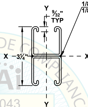
1 5/8 x 1 5/8 x 12ga DOUBLE STRUT
