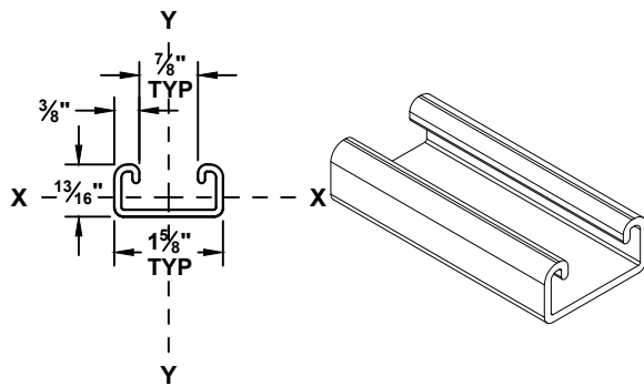
13/16 x 1 5/8 x 12ga SINGLE STRUT
