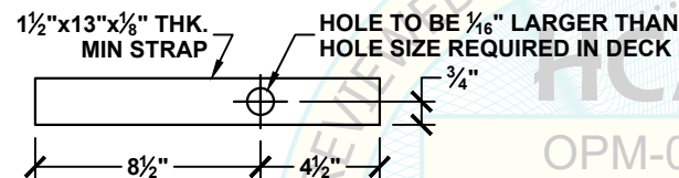
INSERT PLACEMENT STRAP
