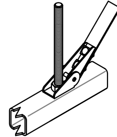
TRANSVERSE BRACING
