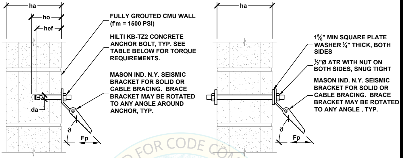
DETAIL FOR UNCRACKED CONDITIONS
