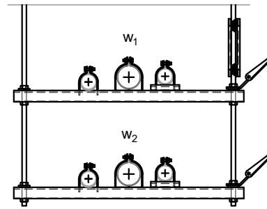
CASE 2 IF w_1 \geq 10 LB/FT AND w_2 \geq 10 LB/FT, BRACE EACH LAYER INDEPENDENTLY
