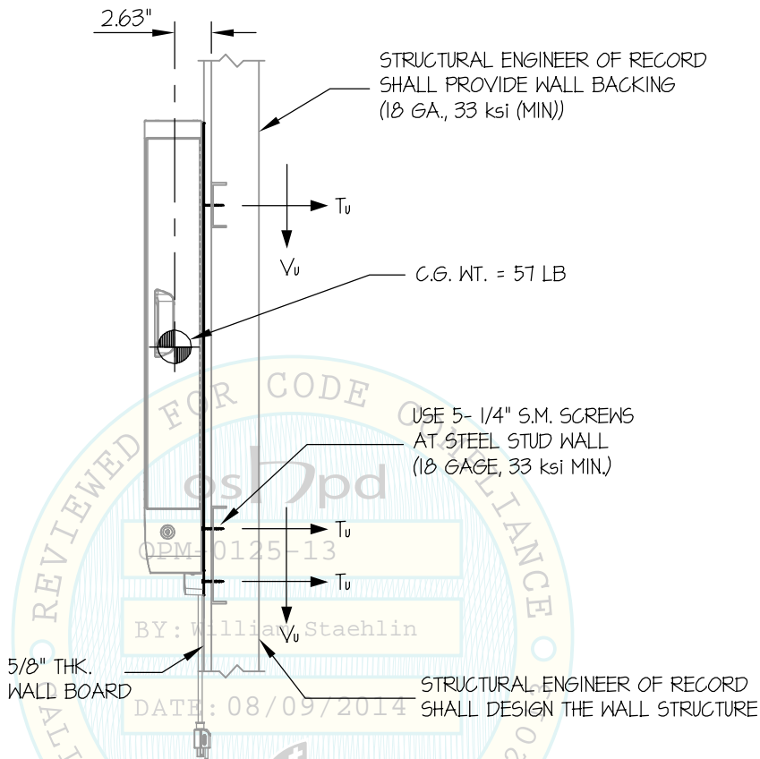
STEEL STUD WALL SECTION (TABLE MANAGEMENT)
