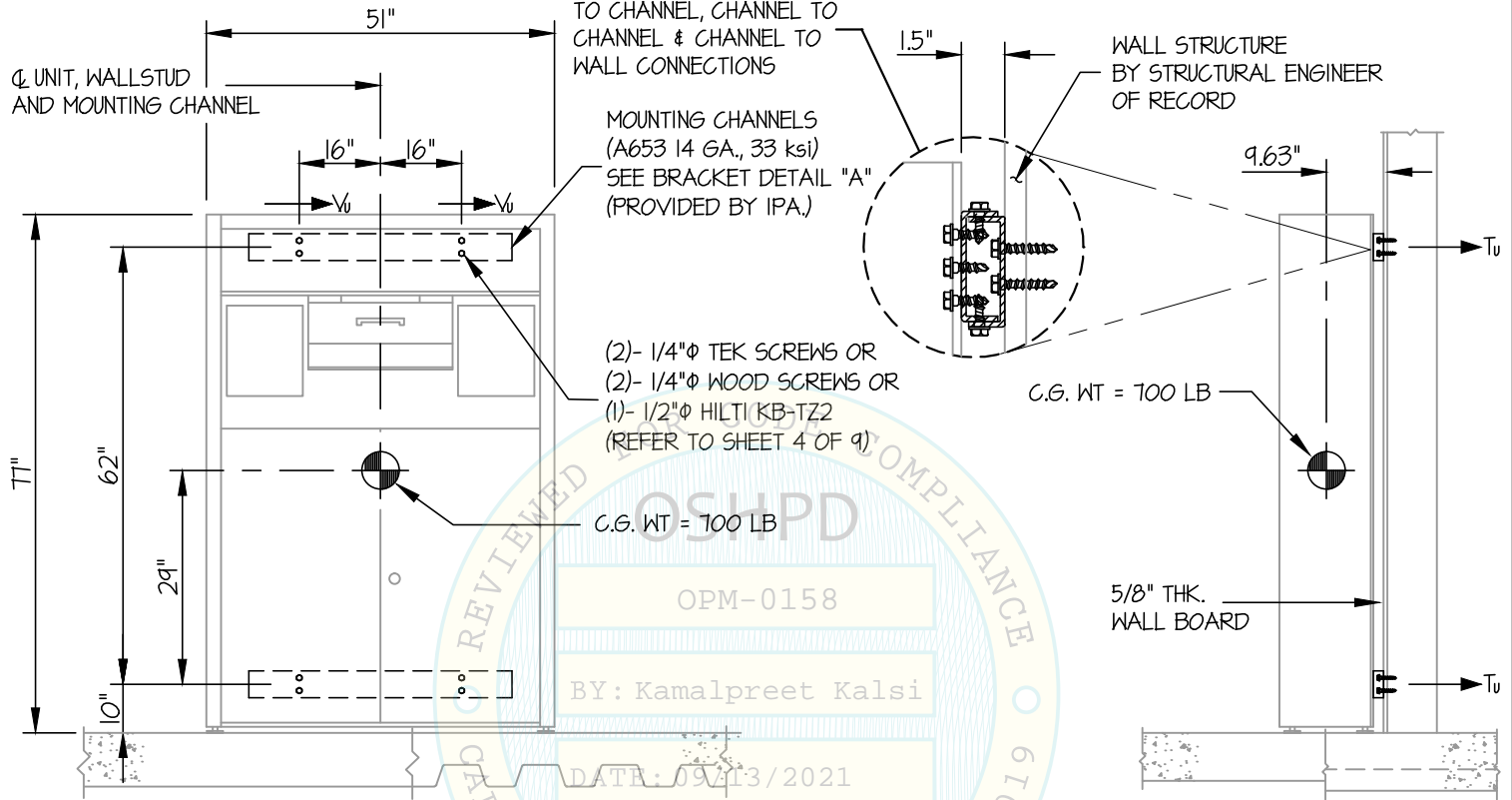
FRONT ELEVATION
