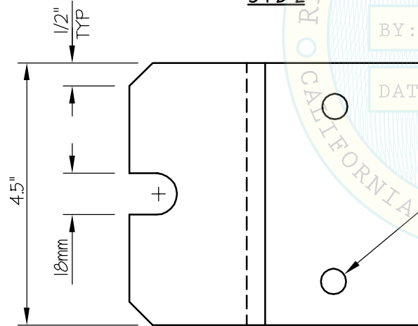
PLAN AT BRACKET
