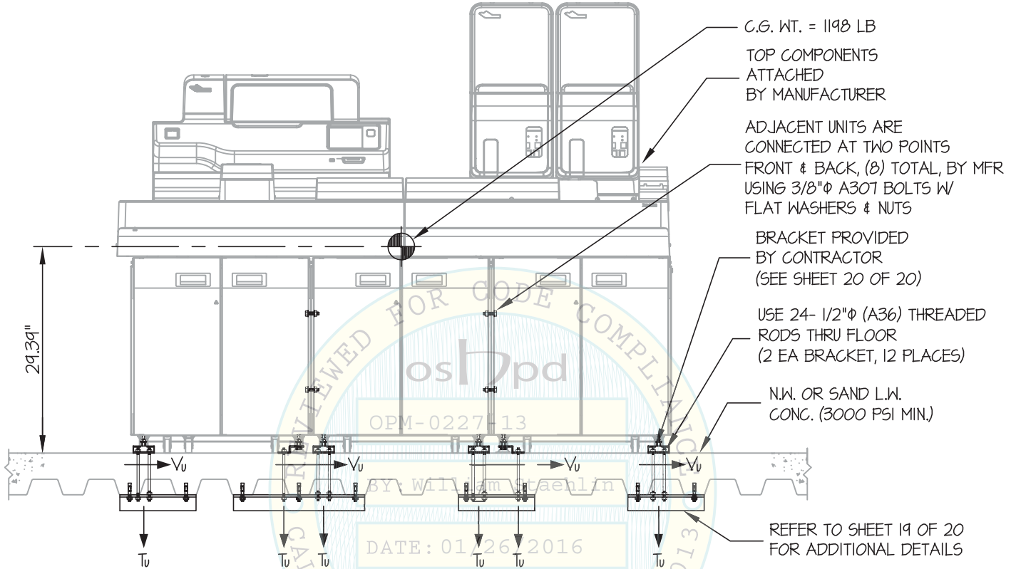
FRONT ELEVATION (XN-3000 + WG-II MODEL)
