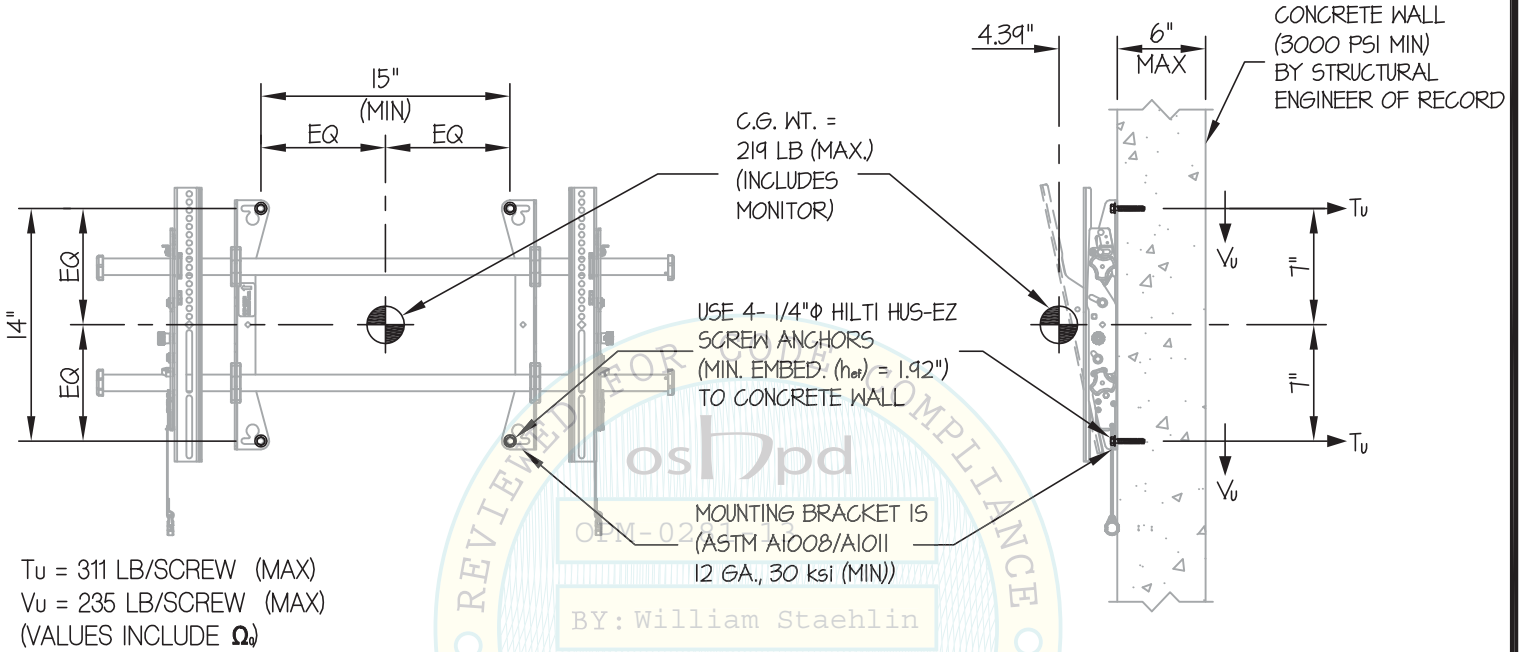
ELEVATION AT WALL PLATE (LTAIU MODEL SHOWN) CONCRETE WALL SECTION (LTAIU MODEL SHOWN)
