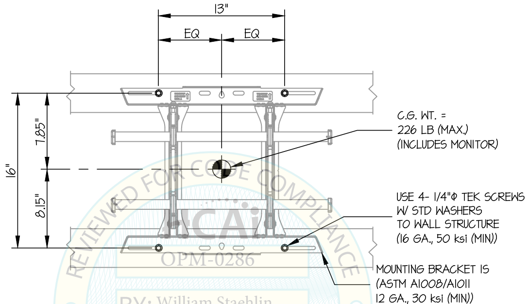
ELEVATION AT WALL PLATE (MTMP1U MODEL SHOWN)
