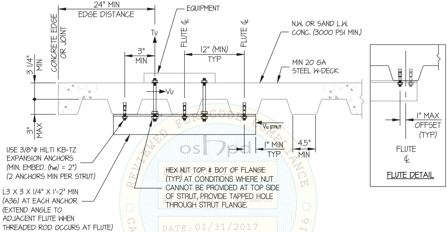
MIN STEEL DECK REQUIREMENTS AND STRUT DETAIL (ALTERNATE MOUNTING CONFIGURATION) (A)
