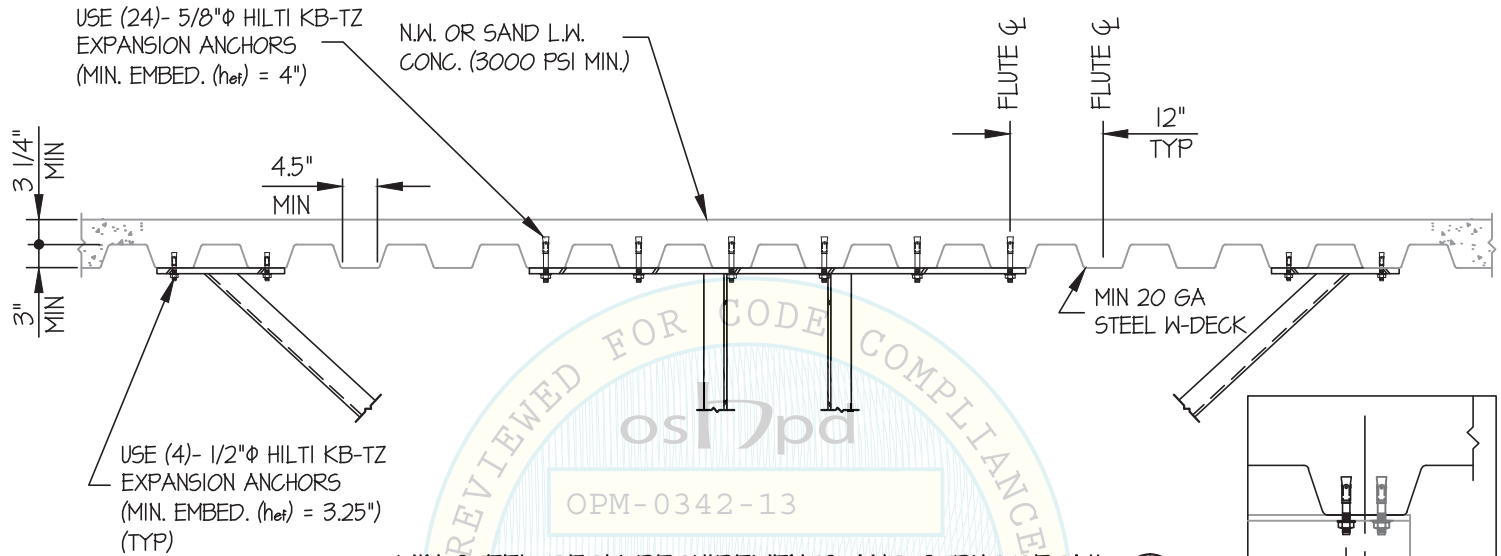
MIN STEEL DECK REQUIREMENTS AND STRUT DETAIL (E)
