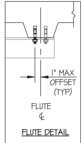
MIN STEEL DECK REQUIREMENTS AND STRUT DETAIL (E)
