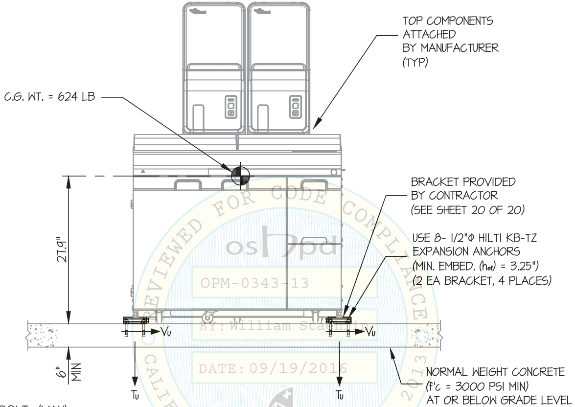
FRONT ELEVATION (XN-9100 (CV-55) MODEL)
