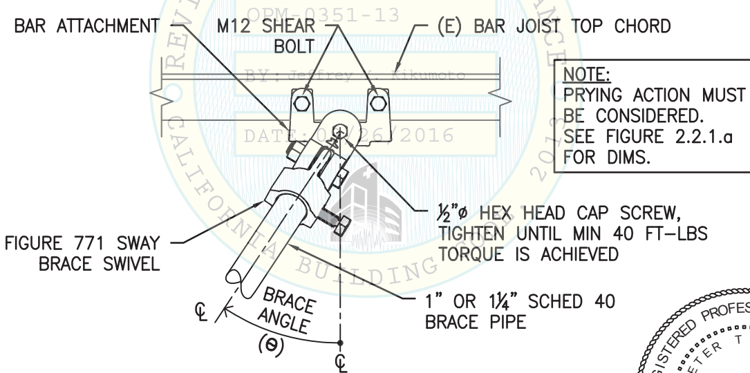
FIGURE 4.3.5 – FIGURE 778 & FIGURE 771 VERT ORIENTATION, FRONT VIEW
