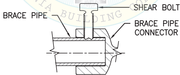
FIGURE 5.2.2 – SHEAR BOLT-BRACE PIPE INTERACTION DETAIL
