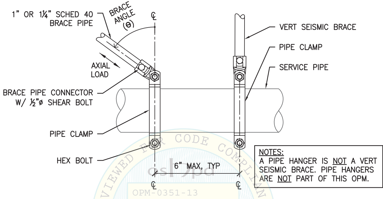
FIGURE 5.2.3 – LONG & VERT SEISMIC BRACE ORIENTATION
