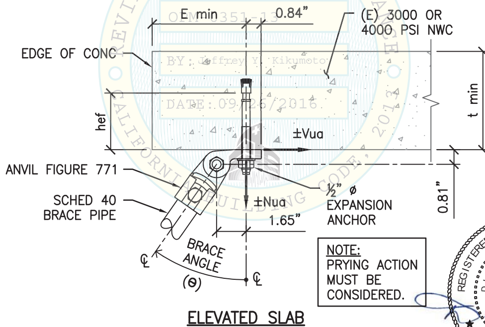
FIGURE 2.2.1a – ANCHORING DETAILS FOR 3000 PSI & 4000 PSI NWC
