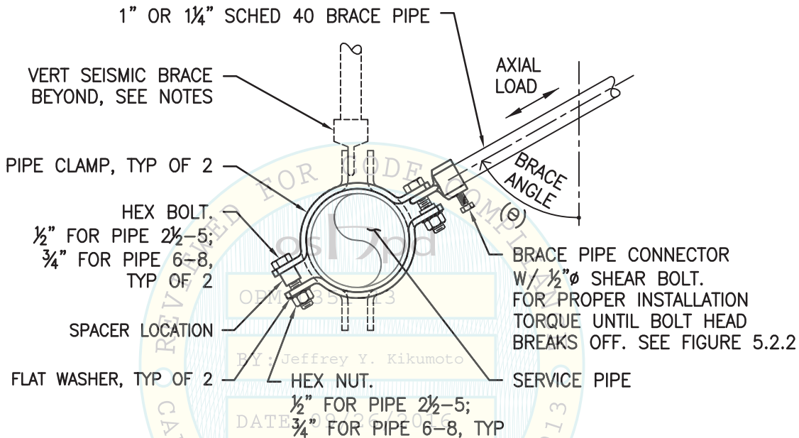
FIGURE 5.2.1 – TRANS & VERT SEISMIC BRACE ORIENTATION
