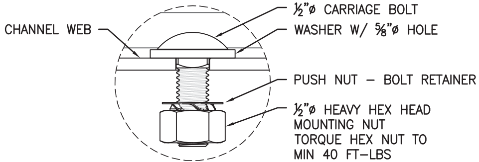
FIGURE 4.2.3 – DETAIL OF CARRIAGE BOLT ASSEMBLY
