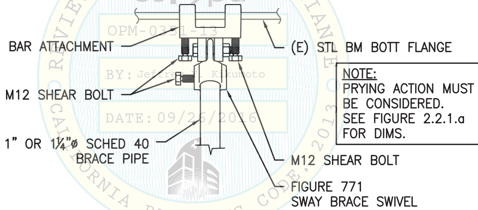
FIGURE 4.3.3 – FIGURE 778 & FIGURE 771 HORIZ ORIENTATION, FRONT VIEW
