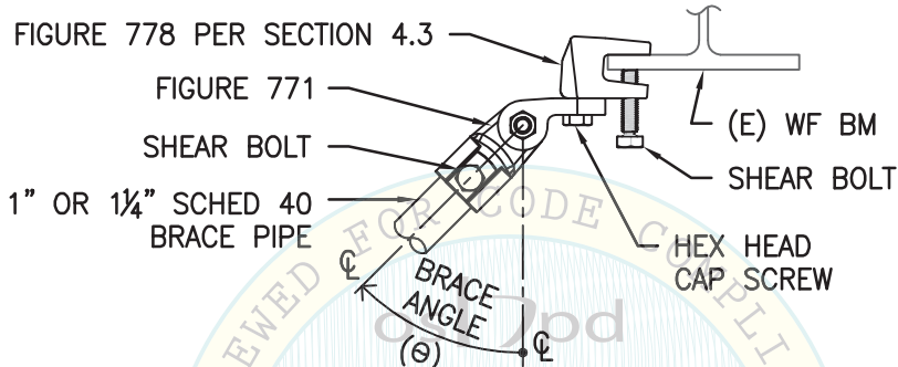
FIGURE 4.1.4 – EXAMPLE OF FIGURE 771 CONNECTED TO FIGURE 778 BM CLAMP
