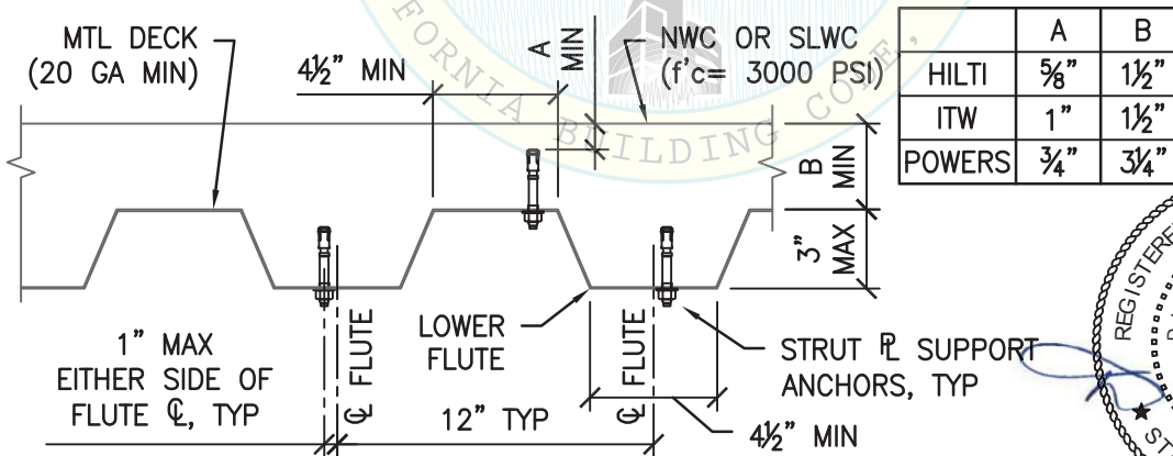
FIGURE 2.1.2 - ANCHOR IN SOFFIT OF MTL DECK
