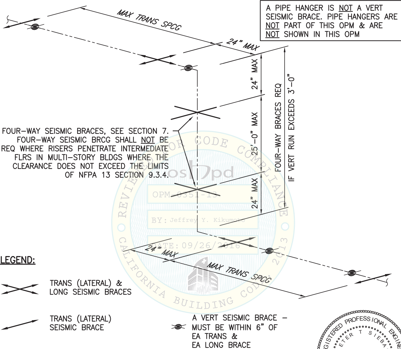
FIGURE 1.2.4 – BRCG FOR PIPING W/ A VERT RISER
