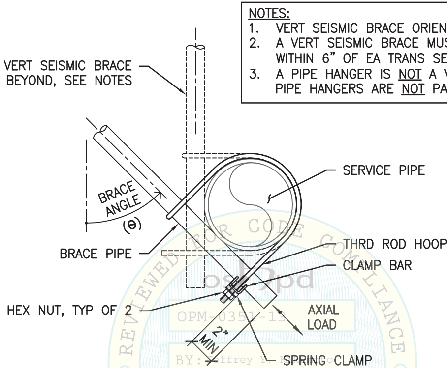
FIGURE 5.1.2 – TRANS & VERT SEISMIC BRACE ORIENTATION OPM-0351-13 BY: Jeffrey Kikumoto DATE: 09/26/2016
