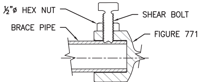
FIGURE 4.1.3 – SHEAR BOLT – BRACE PIPE INTERACTION DETAIL
