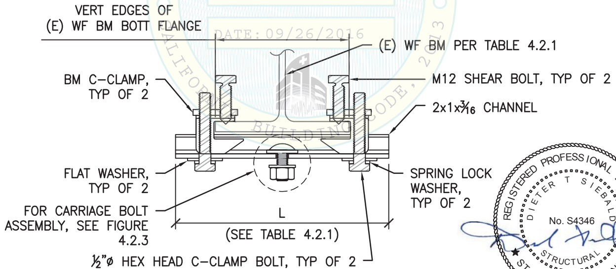
FIGURE 4.2.2 – SECTION VIEW OF FIGURE 772
