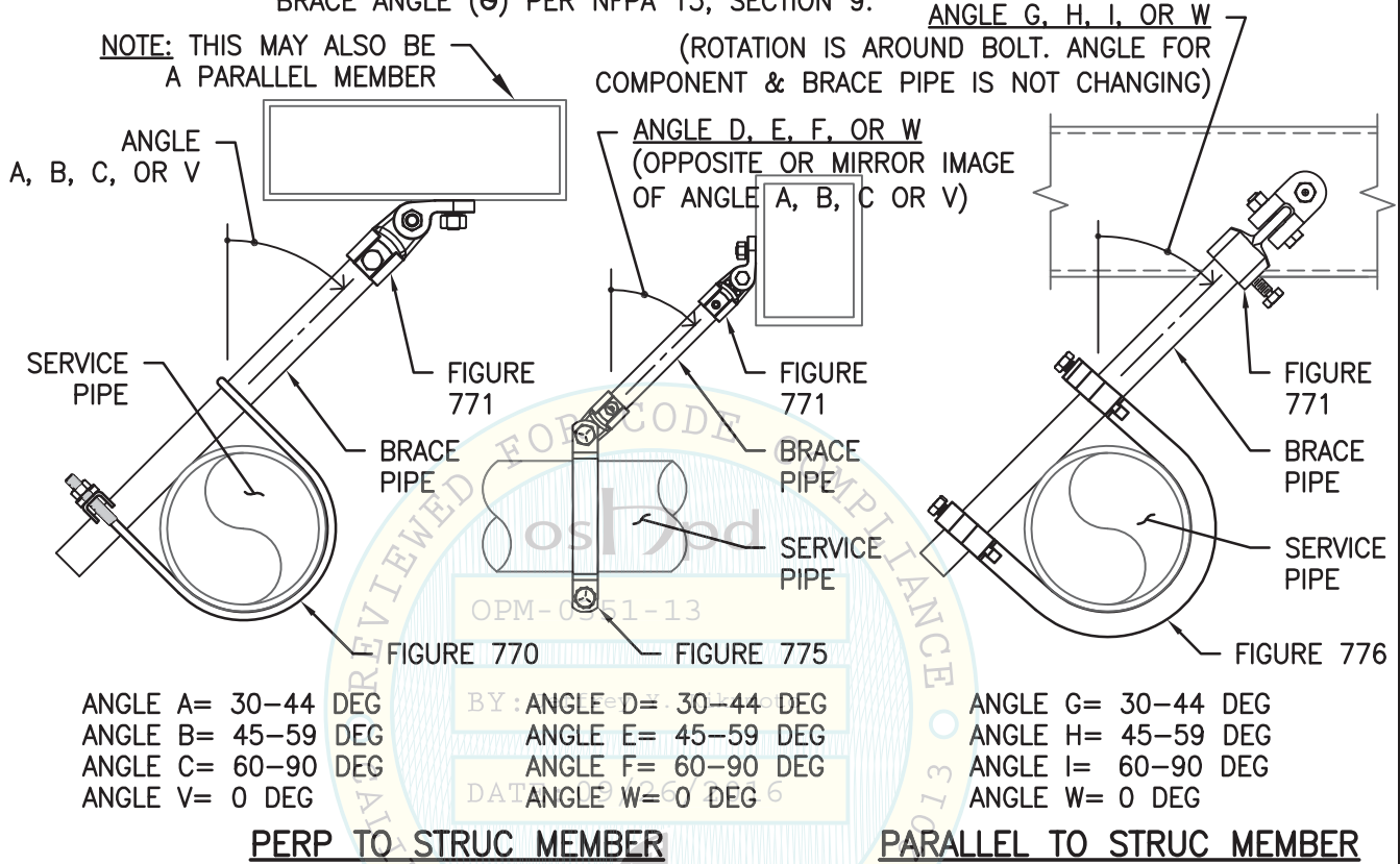
FIGURE 4.1.2 – FIGURE 770, FIGURE 775, & FIGURE 776
