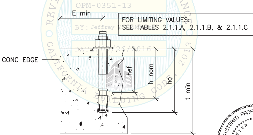
FIGURE 2.1.1 - ANCHOR INSTALLATION INFO
