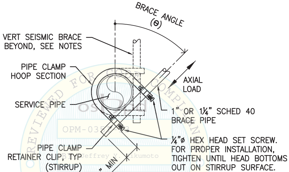
FIGURE 5.3.1 – TRANS & VERT SEISMIC BRACE ORIENTATION
