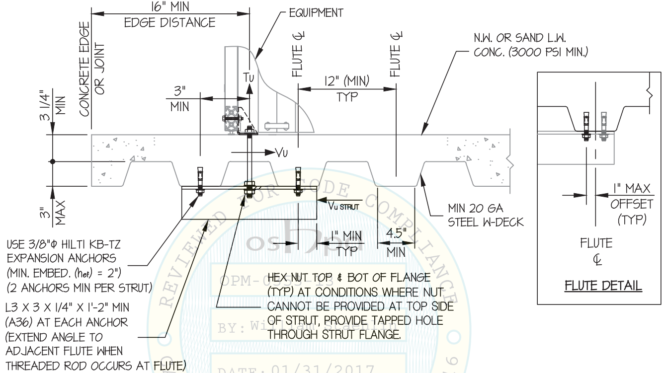
MIN STEEL DECK REQUIREMENTS AND STRUT DETAIL (B)
