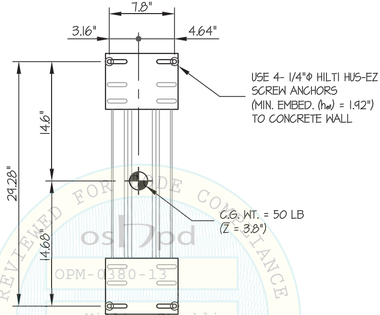
ELEVATION AT WALL PLATE
