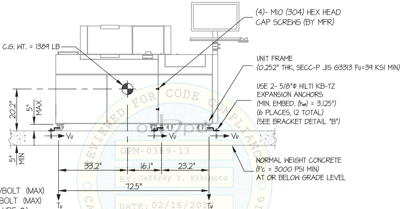
FRONT ELEVATION (ANL & SMP)
