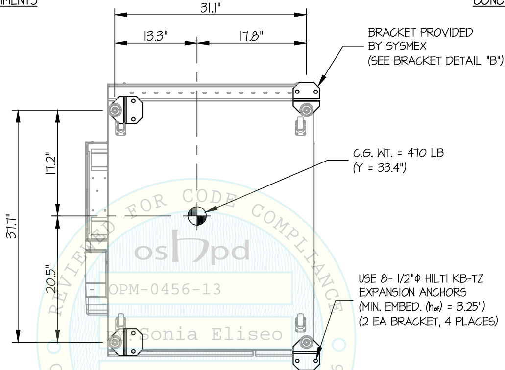
PLAN AT BASE (XN-3100 (DI-60+CF-70+WG-80) MODEL)
