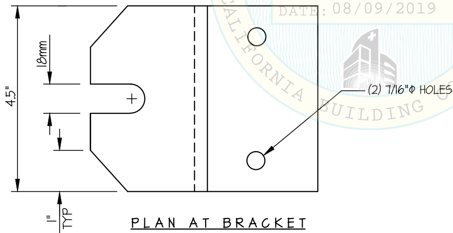
BRACKET DETAIL (B)
