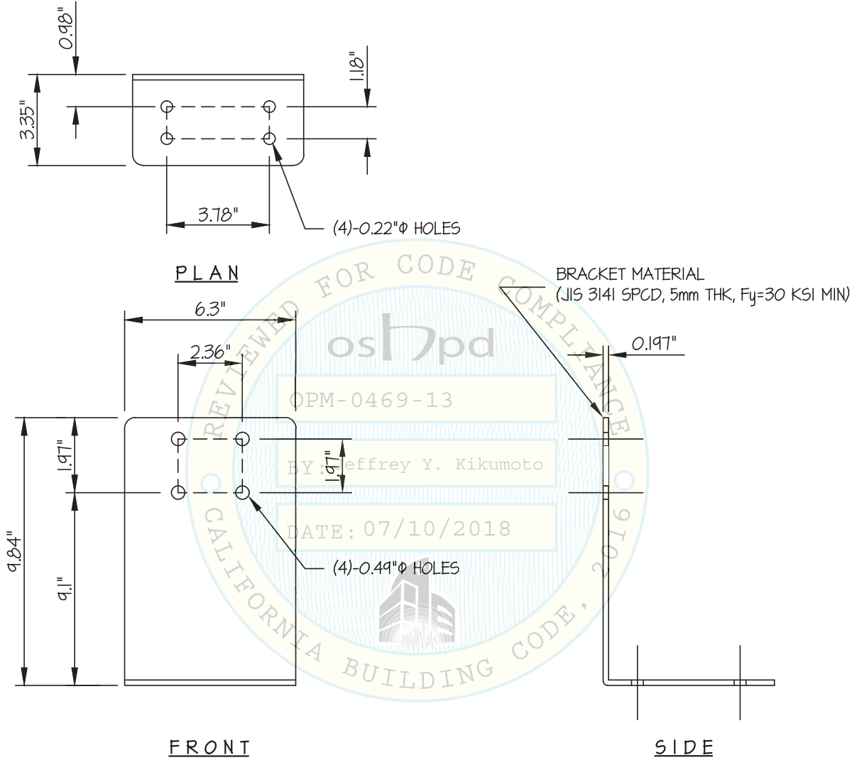
BRACKET TO UNIT DETAIL (B)
