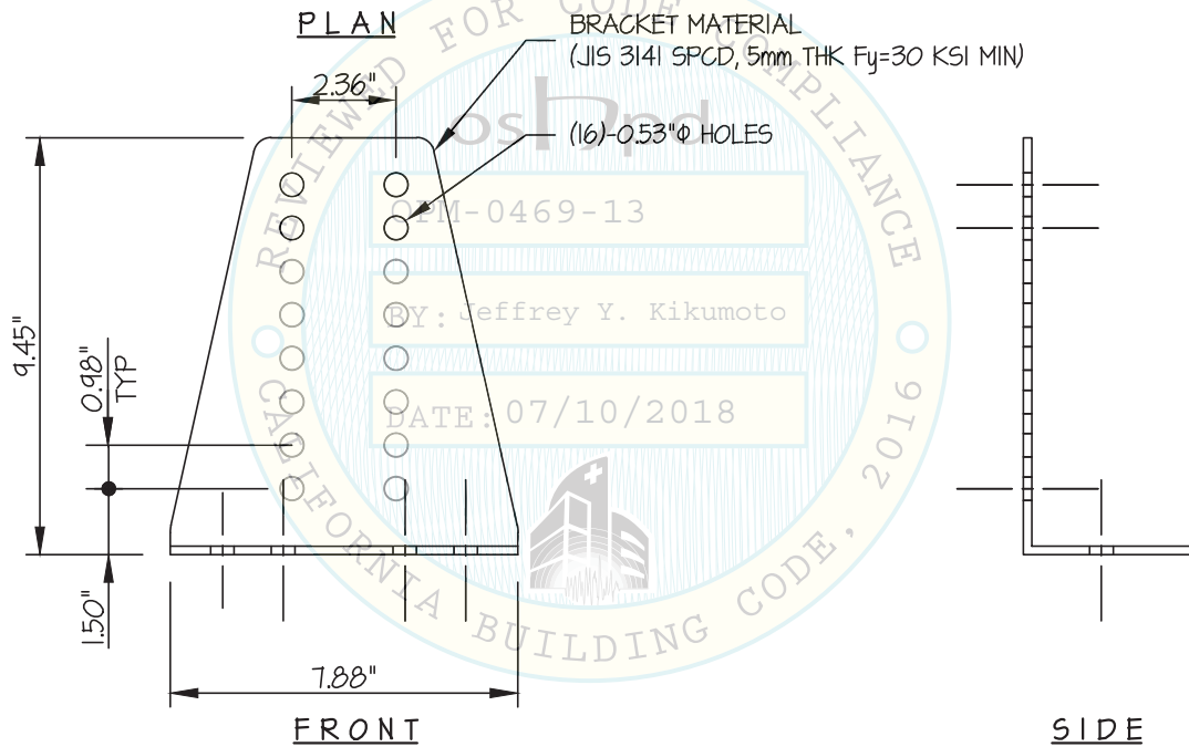
WALL BRACKET DETAIL (C)
