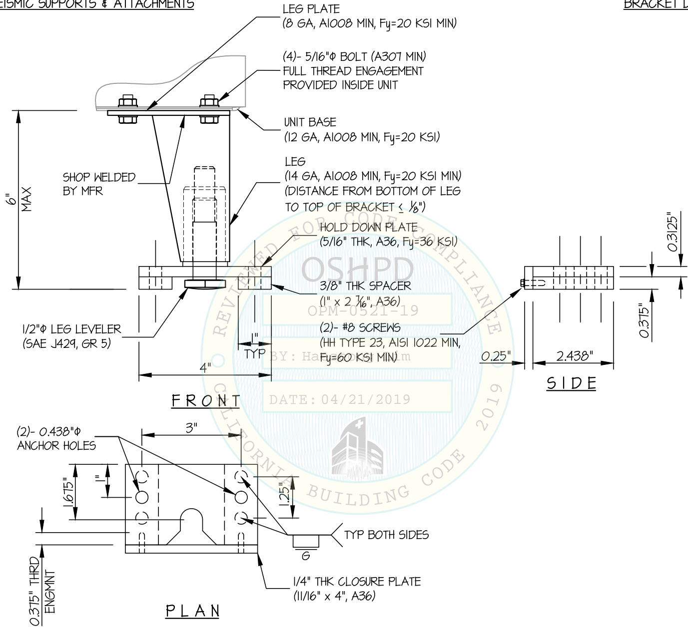
BRACKET DETAIL (B)
