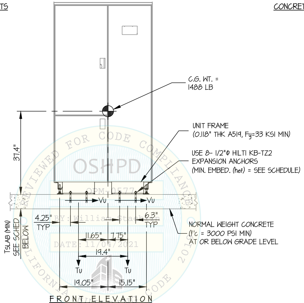
FRONT ELEVATION
