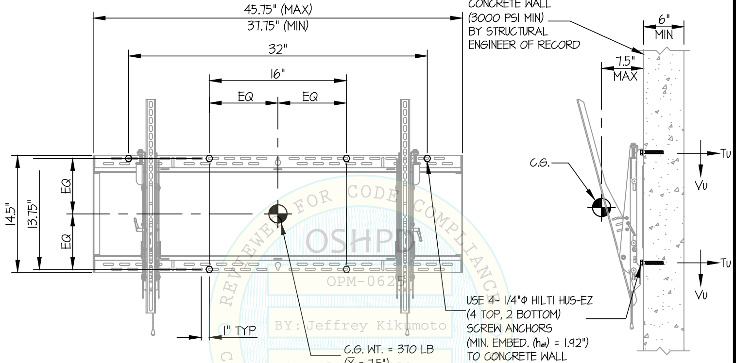
CONCRETE WALL SECTION
