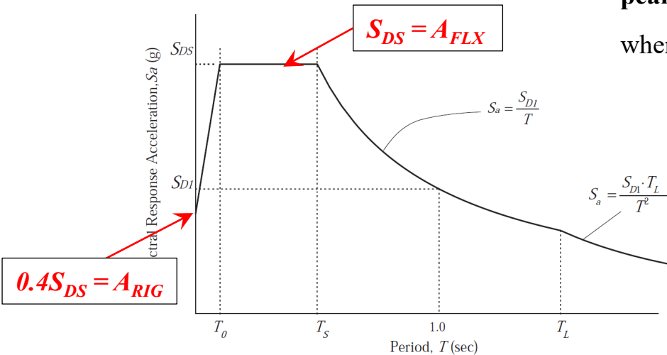
Figure 11.4-1. Two-period design response spectrum.
