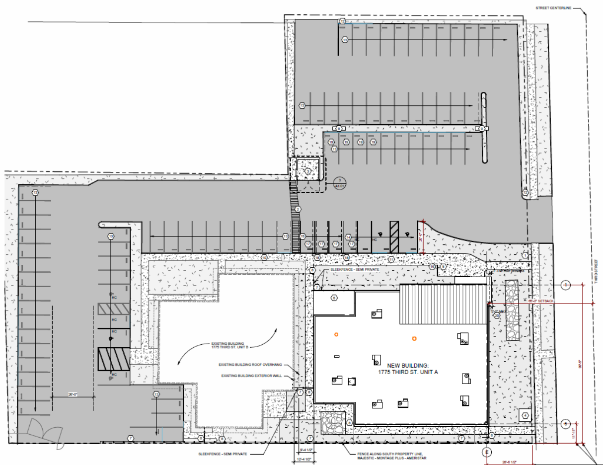
Site Plan
