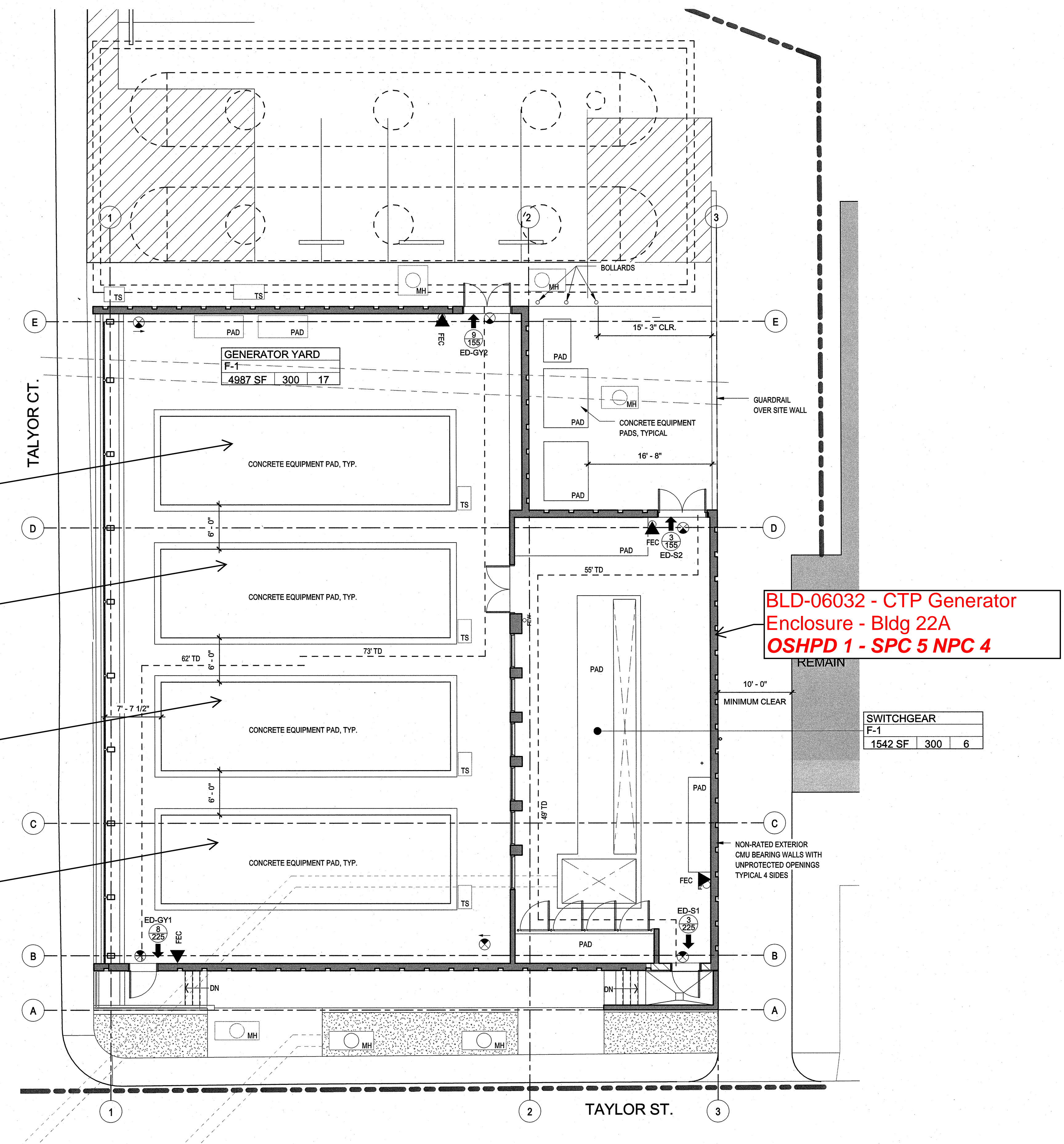
① LIFE SAFETY PLAN 1/8" = 1'-0"
