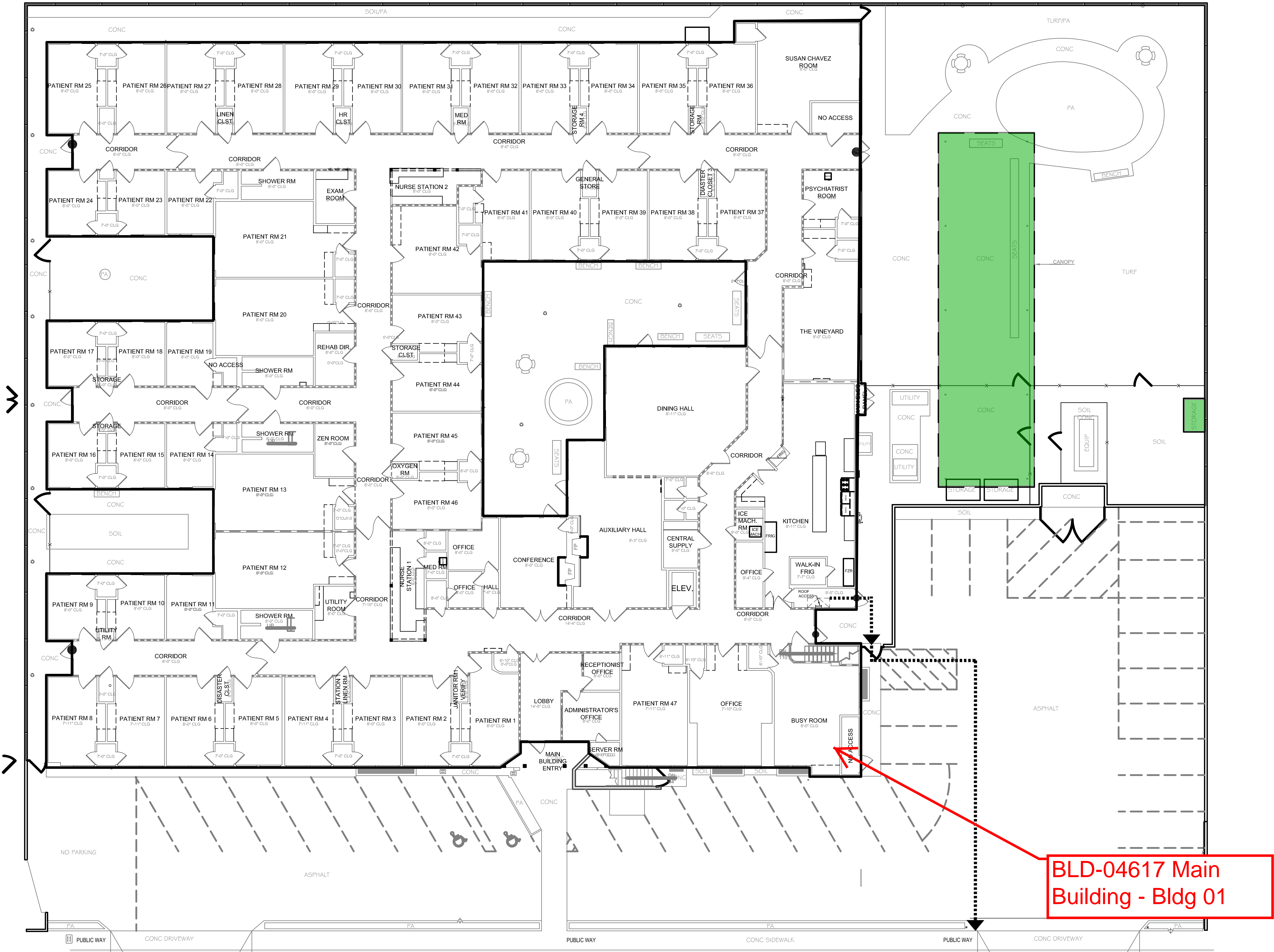
1 SITE PLAN / GROUND FLOOR EGRESS PLAN SCALE : 3/32" = 1'-0"
