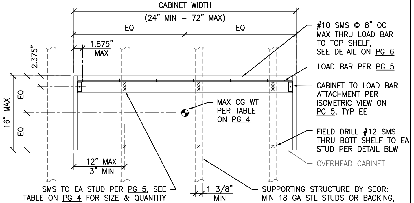
FRONT ELEV
