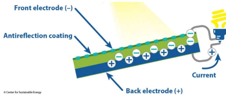
Figure 4. The Photoelectric Effect (GO Solar California).
