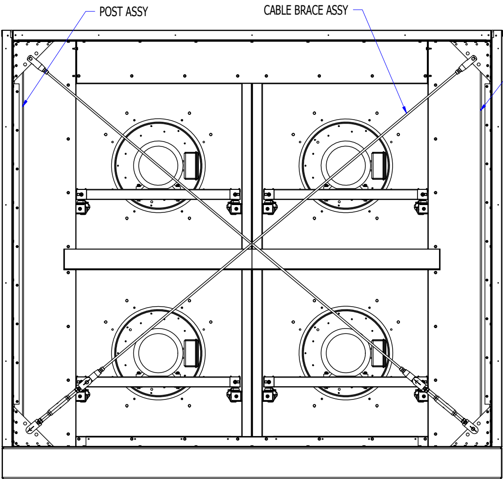
DISCHARGE VIEW
