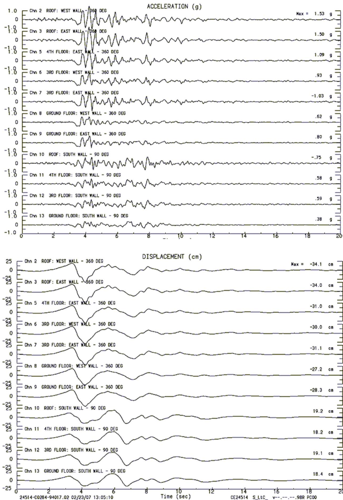
Figure 8. Structural responses (accelerations at the top and displacements at the bottom) recorded by seismic instrumentation system installed at the new Sylmar County Hospital during the 1994 Northridge earthquake 6 .
